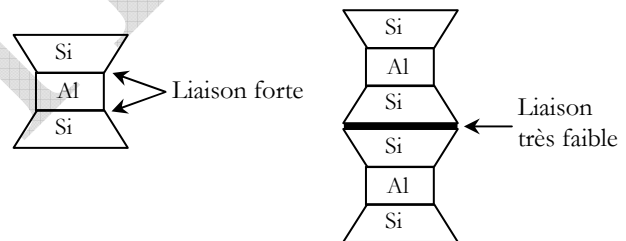
Figure 2.20 : Montmorillonite
