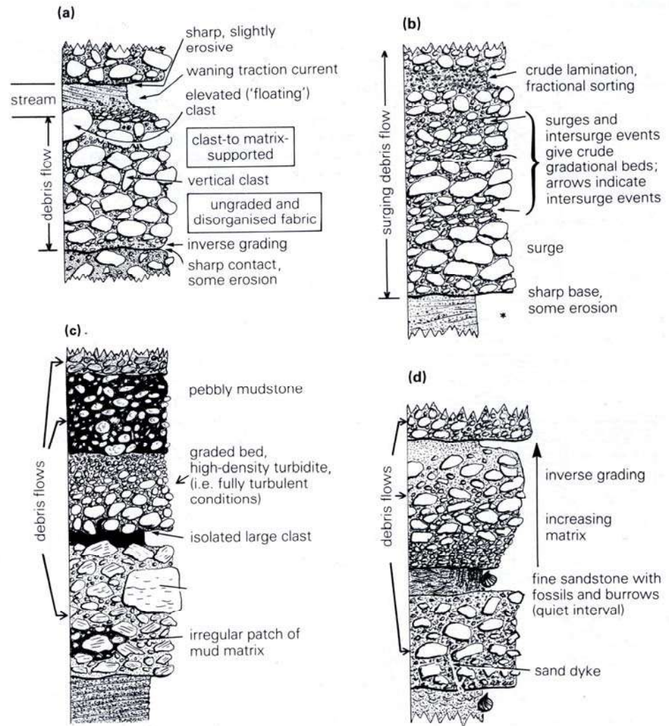
Examples of different styles of grading in conglomerates due to different depositional processes acting in a variety of typical sub-aerial (a,b) and sub-aqueous settings (c,d). Bed thickness ranges from a few decimetres to metres (after Nemec & Steel 1984, Figs 15 & 16).
