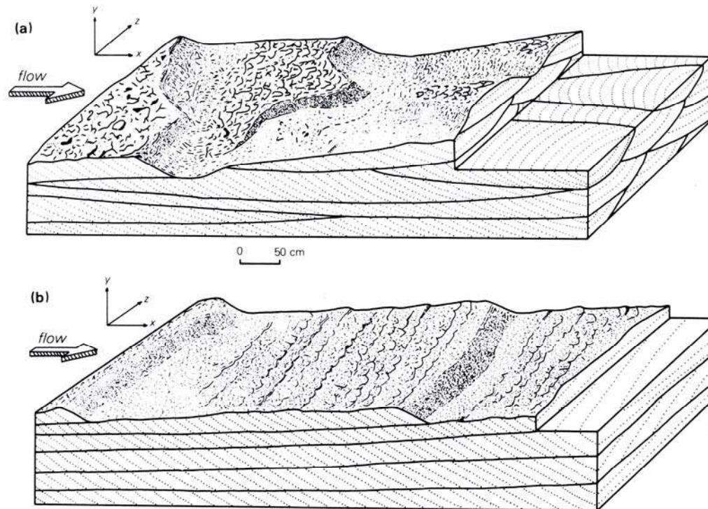
Patterns of cross bedding generated by the migration of: (a) dunes (trough cross bedding; see Fig. 6.31a) and (b): sandwaves (tabular cross bedding; see Fig. 6.31c). (After Harms et al. 1975.)
