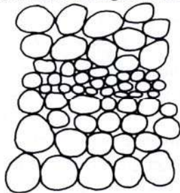
(b) Orthoconglomerate
