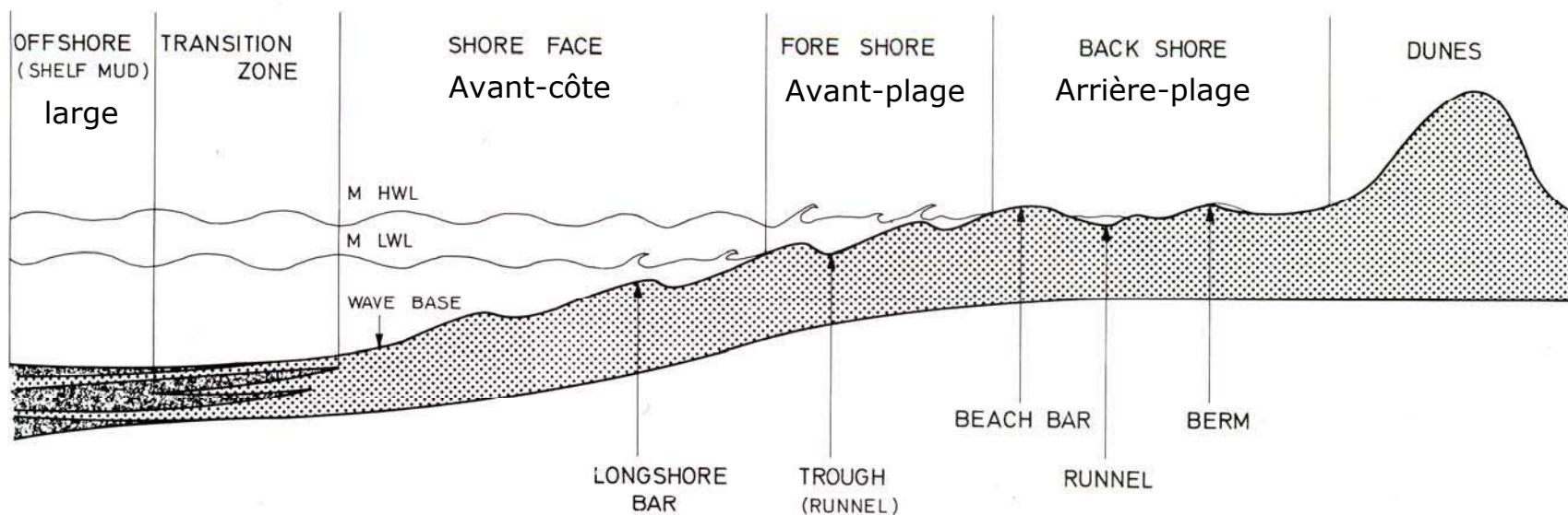
Fig. 410 Schematic representation of the terminology of the various geomorphic units of a beach profile. Various geomorphic features of a beach as well as transition to shelf mud are shown. The terminology is mainly based on EMERY (1960a)
