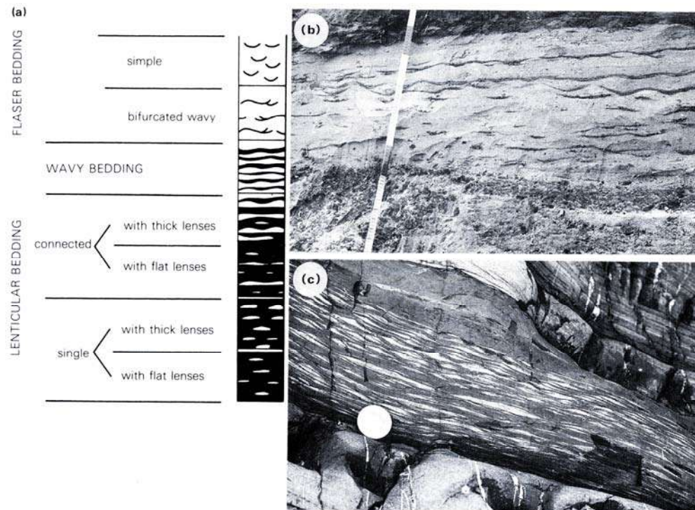
(a) The variety of cross lamination resulting from mixed lithologies of sand and mud (after Reineck and Singh 1973). Photographs illustrate: (b) flaser bedding with mud drapes predominantly in the ripple troughs (Haringvliet excavation, Netherlands); (c) lenticular bedding with rather peaked symmetrical ripple form sets. (Northam Formation, Upper Carboniferous, North Devon.)
