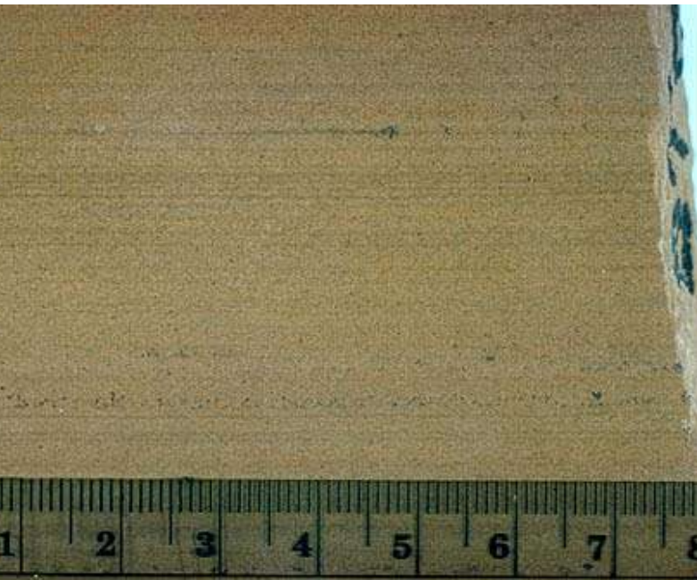
Polished slab of typical, finely laminated, very fine-grained basinal sandstone_siltstone
