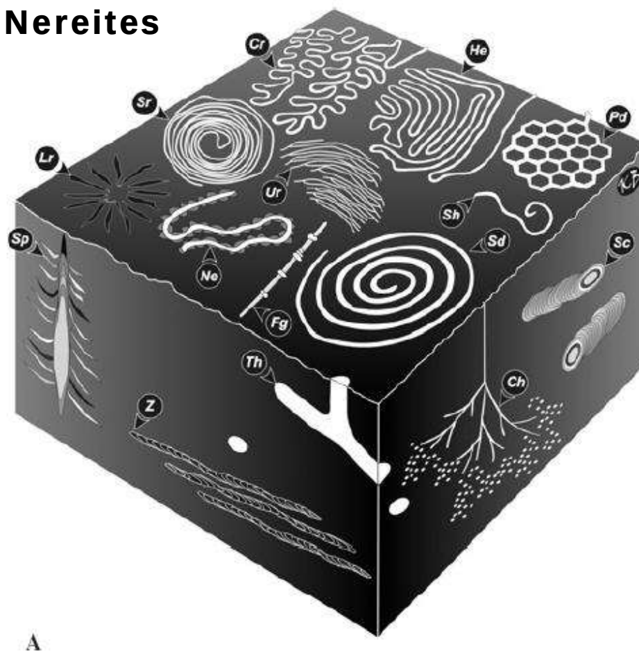
FIGURE 4.7 The Nereites Ichnofacies. (A) Diagram of the Nereites Ichnofacies. Traces include Chondrites (Ch), Cosmorhapse (Cr), Fustiglyphus (Fg), Helminthorhapse (He), Lorenzina (Lr), Nereites (Ne), Paleodictyon (Pd), Planolites , Scolicia (Sc), Spirodesmos (Sd), Spirophycus (Sh), Spirophyton (Sp), Spirorhapse (Sr), Thalassinoides (Th), Urohelminthoida (Ur), and Zoophycos (Z). (B) Bedding plane of Scolicia (arrows), Upper Cretaceous Nanaimo Group, British Columbia. (C) Thin, muddy Zoophycos (Z), with Helminthopsis (H), and Cosmorhapse (Cr), Upper Cretaceous, North Slope of Alaska. (D) Bedding plane entirely covered with Nereites , Eocene Zumaya Flysch, Spain. (E) Bedding plane with abundant Nereites , Eocene, Austria. (F) Paleodictyon cast on the sole of a thin turbidite bed, Eocene Zumaya Flysch, Spain. (G) Spirorhapse cast on the sole of a thin turbidite bed, Eocene, Austria.
