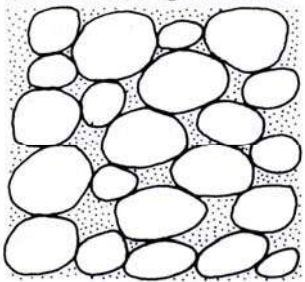
(a) Orthoconglomerate
