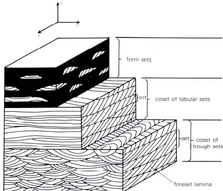
Definition diagram for the basic types of cross lamination. The same terms apply at a larger scale to cross bedding (based on Allen 1968).
