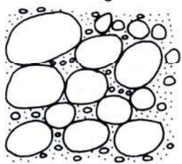
(c) Orthoconglomerate
