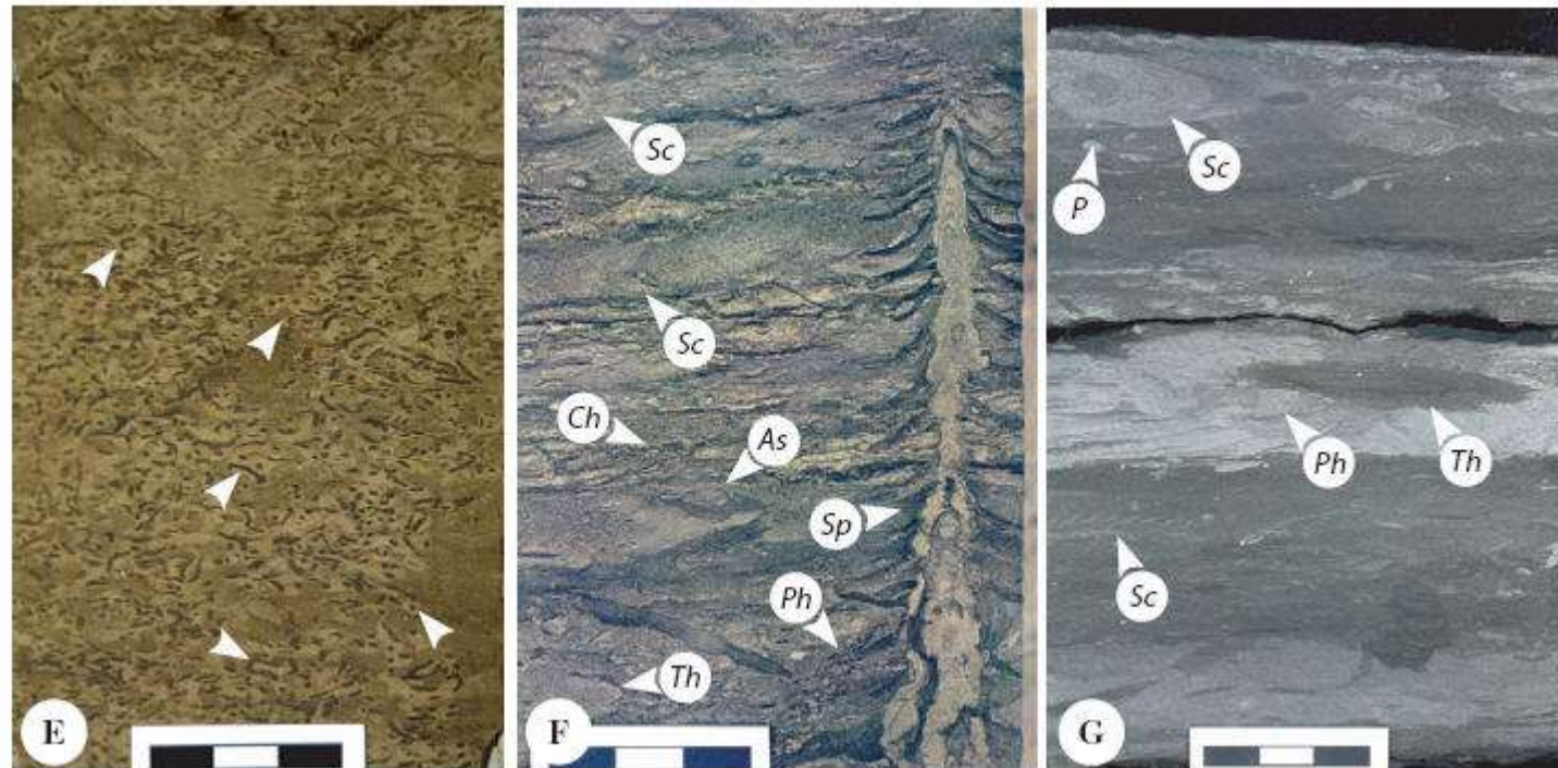
FIGURE 4.6 The Zoophycos Ichnofacies. (A) Diagram of the Zoophycos Ichnofacies. Traces include Chondrites (Ch), Cosmorhapse (Cr), Phycosiphon (Ph), Planolites (P), Scolicia (Sc), Spirophyton (Sp), Thalassinoides (Th), and Zoophycos (Z). (B) Abundant Zoophycos (Z) and Planolites (P), Upper Cretaceous Doe Creek Formation, Alberta. (C) Zoophycos (Z), Helminthopsis (H), and Cosmorhapse (Cr) in shelf deposits, Upper Cretaceous, Northern North Sea, Norway. (D) Zoophycos (Z) structure from slope deposits of the Upper Cretaceous Cedar District Formation, British Columbia. (E) Abundant Phycosiphon (arrows) in a shelf diatomite, Miocene Monterey Formation, San Joaquin Basin, California. (F) Scolicia (Sc), Spirophyton (Sp), Chondrites (Ch), Phycosiphon (Ph), Thalassinoides (Th), and diminutive Asterosoma (As) in shelf deposits of the Upper Cretaceous Northern North Sea, Norway. (G) Scolicia (Sc), Planolites (P), Phycosiphon (Ph), and Thalassinoides (Th) from shelf deposits of the Upper Cretaceous San Miguel Formation, Texas.
