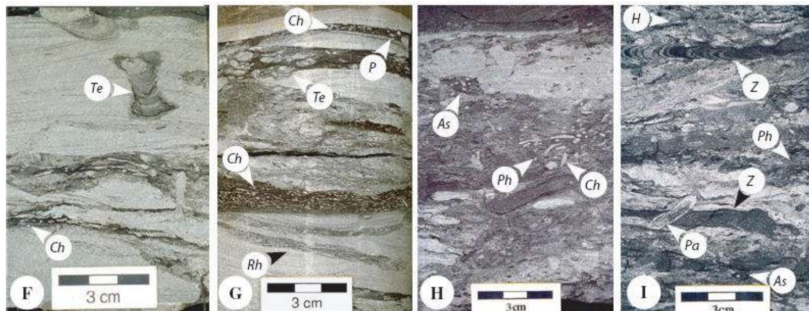
FIGURE 4.5 The Cruziana Ichnofacies. (A) Diagram of the Cruziana Ichnofacies showing the archetypal as well as distal and proximal expressions (artwork by Tom Saunders). (B) Siderite-cemented Rosselia socialis (arrow), Lower Cretaceous Viking Formation, Alberta. (C) Complete Asterosoma (arrow) exposed on bedding plane of outcrop, Upper Cretaceous Cardium Formation, Alberta. (D) Asterosoma lobes (arrows) in outcrop, Upper Cretaceous Blackhawk Formation, Book Cliffs, Utah. (E) Silicified Thalassinoides (arrow) showing Y-shaped branch, Mississippian Mount Head Formation, Mount Greenock, Jasper, Alberta. (F) Storm-bedded upper offshore deposits, with Teichichnus (Te) and Chondrites (Ch), Upper Cretaceous Cardium Formation, Alberta. (G) Heterolithic distal delta front deposits, with dense Chondrites (Ch), small Teichichnus (Te), Planolites (P), and Rhizocorallium (Rh), Lower Cretaceous Bow Island Formation, Alberta. (H) Upper offshore deposits with Asterosoma (As) (reburrowed with Chondrites ), Phycosiphon (Ph), and robust Chondrites (Ch), Upper Cretaceous Cardium Formation, Alberta. (I) Upper offshore deposits with Helminthopsis (H), Zoophycos (Z), Phycosiphon (Ph), Palaeophycus (Pa), and Asterosoma (As), Upper Cretaceous Cardium Formation, Alberta.
