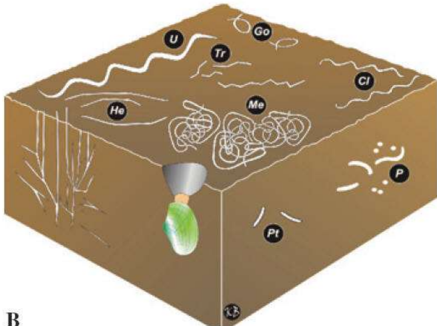
FIGURE 4.2 Schematic block diagrams of continental ichnofacies. (A) Diagram of the Scoyenia Ichnofacies. Traces include Ancorichnus (An), adhesive meniscate burrows (amb), Camborygma (Ca), Cochlichnus (Cl), tetrapod footprints (F), Macanopsis (M), Palaeophycus tubularis (Pt), Planolites (P), rhizoliths (R), Scoyenia (Sc), and Skolithos (S). (B) Diagram of the Mermia Ichnofacies. Traces include bivalve dwellings, Cochlichnus (Cl), Gordia (Go), Helminthoid ichnites (He), Mermia (Me), Planolites (P), Treptichnus (Tr), Palaeophycus tubularis (Pt), and Undichna (U). (C) Diagram of the Coprinisphaera Ichnofacies. Traces include Celliforma (Ce), Coprinisphaera (Co), Eatonichnus (Ea), footprints (F), roots (Rt), Skolithos (S), adhesive meniscate burrows (amb), Teisseirei (Ti), and Termitichnus (Tm). (D) Scratch-marked expression of Scoyenia (Sc), with meniscate visible in the right-hand example, Triassic Tarkastad Subgroup, Karoo Basin, South Africa. (E) Adhesive meniscate burrows (amb), Lower Cretaceous Mannville, Group, Alberta, Canada. (F) Modern Undichna (U), formed by the pectoral fins of fish, and tetrapod footprints (F) in mud, Australia. (G) Gordia (Go), Upper Permian Balfour Formation, Karoo Basin, South Africa. (H) Termitichnus (Tm), Pleistocene of the Karoo Basin, South Africa. Photo (D) courtesy of Dr. Fiona J. Evans.
