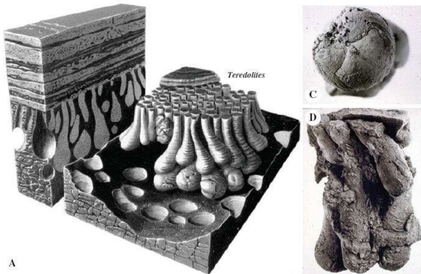
FIGURE 4.9 The Teredolites Ichnofacies. (A) Diagram of the Teredolites Ichnofacies (artwork by Tom Saunders). (B) Teredolites clavatus (white arrow) in peat horizon, truncated by mud-filled channel (black arrow), Upper Cretaceous Horseshoe Canyon Formation, Drumheller. (C) The wood-boring bivalve Martesia sp. at the base of the Teredolites clavatus depicted in (B) and (D). (D) Teredolites clavatus from the horizon depicted in (B) and (C). (E) Siderite-cemented Teredolites clavatus , Upper Cretaceous Horseshoe Canyon Formation, Drumheller. (F) Woodground Thalassinoides ( Th ), at the base of a tidal channel excavated into coal, Upper Cretaceous Ferron Sandstone, Utah. (G) Teredolites (arrows) excavated into lignitic coal, Lower Cretaceous Grand Rapids Formation, Alberta.
