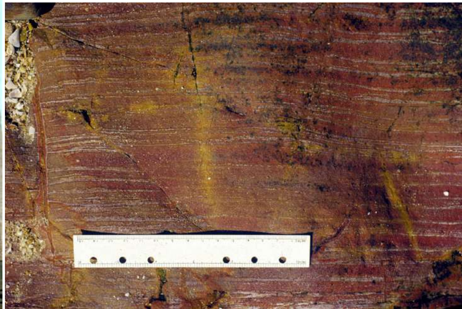
Finely laminated siltstone and fine-grained sandstone, of the Carboniferous, Mai Po Member
