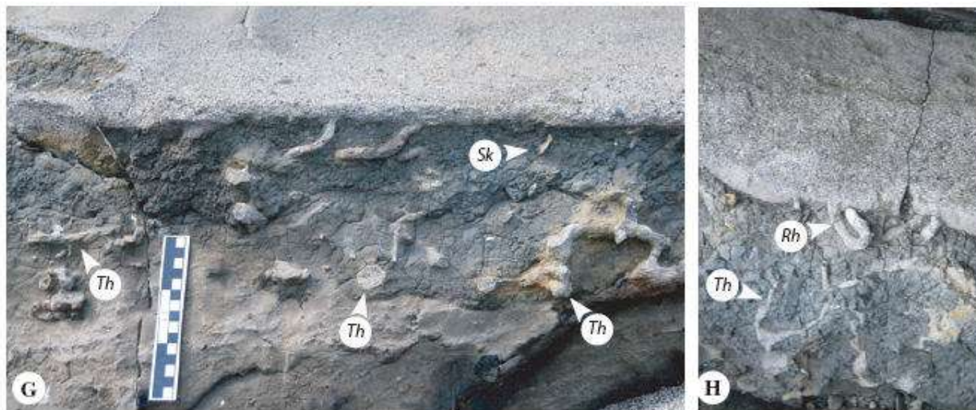
FIGURE 4.8 The Glossifungites Ichnofacies. (A) Diagram of the Glossifungites Ichnofacies. Firmground ichnogenera include Skolithos (S), Gastrochaenolites (G), Arenicolites (A), Diplocraterion (D), Psilonichnus (Ps), Conichnus (C), Bergaueria (B), Palaeophycus (P), Taenidium (Ta), Rhizocorallium (Rh), Thalassinoides (Th), Chondrites (Ch), and Zoophycos (Z). (B) Firmground Skolithos cross-cutting offshore mudstone and subtending from an amalgamated sequence boundary and flooding surface, Lower Cretaceous Viking Formation, Alberta. (C) Firmground Arenicolites filled with coarse-grained sandstone, associated with a transgressive surface of erosion, Lower Cretaceous Viking Formation, Alberta. (D) Firmground Thalassinoides subtending from an incised valley complex, Upper Cretaceous Dunvegan Formation, Alberta. (E) Firmground Rhizocorallium subtending from the base of an estuarine incised valley complex, Lower Cretaceous Viking Formation, Alberta. (F) Firmground Diplocraterion associated with a transgressive surface of erosion, Jurassic Gravelburg Formation, Saskatchewan. (G) Submarine canyon margin with a firmground suite of Thalassinoides (Th), and Skolithos (Sk), lower Miocene Nihotupu and Tirikohua formations, Northland, New Zealand. (H) Firmground Rhizocorallium (Rh) and Thalassinoides (Th) demarcating the same discontinuity as shown in (G).
