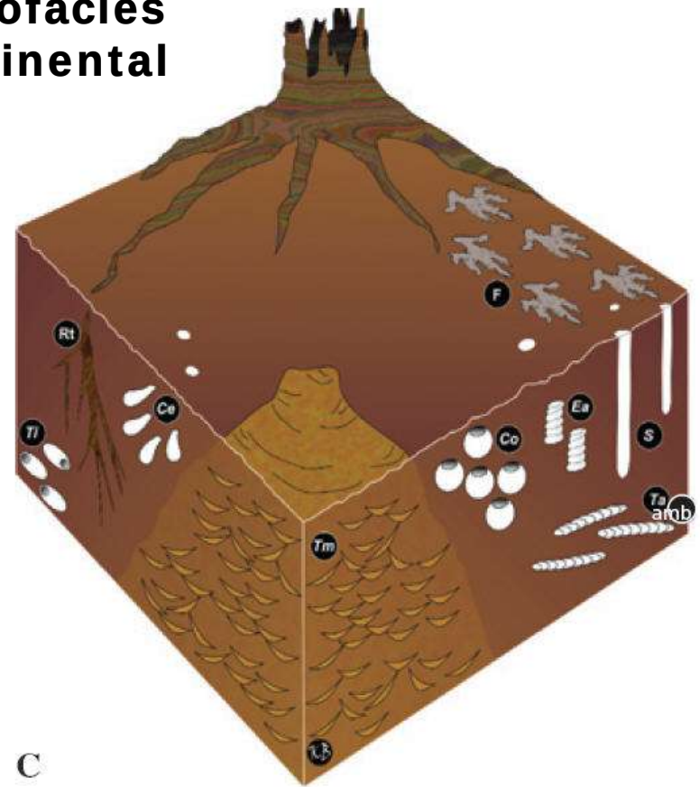
FIGURE 4.2 Schematic block diagrams of continental ichnofacies. (A) Diagram of the Scoyenia Ichnofacies. Traces include Ancorichnus (An), adhesive meniscate burrows (amb), Camborygma (Ca), Cochlichnus (Cl), tetrapod footprints (F), Macanopsis (M), Palaeophycus tubularis (Pt), Planolites (P), rhizoliths (R), Scoyenia (Sc), and Skolithos (S). (B) Diagram of the Mermia Ichnofacies. Traces include bivalve dwellings, Cochlichnus (Cl), Gordia (Go), Helminthoid ichnites (He), Mermia (Me), Planolites (P), Treptichnus (Tr), Palaeophycus tubularis (Pt), and Undichna (U). (C) Diagram of the Coprinisphaera Ichnofacies. Traces include Celliforma (Ce), Coprinisphaera (Co), Eatonichnus (Ea), footprints (F), roots (Rt), Skolithos (S), adhesive meniscate burrows (amb), Teisseirei (Ti), and Termitichnus (Tm). (D) Scratch-marked expression of Scoyenia (Sc), with meniscate visible in the right-hand example, Triassic Tarkastad Subgroup, Karoo Basin, South Africa. (E) Adhesive meniscate burrows (amb), Lower Cretaceous Mannville, Group, Alberta, Canada. (F) Modern Undichna (U), formed by the pectoral fins of fish, and tetrapod footprints (F) in mud, Australia. (G) Gordia (Go), Upper Permian Balfour Formation, Karoo Basin, South Africa. (H) Termitichnus (Tm), Pleistocene of the Karoo Basin, South Africa. Photo (D) courtesy of Dr. Fiona J. Evans.
