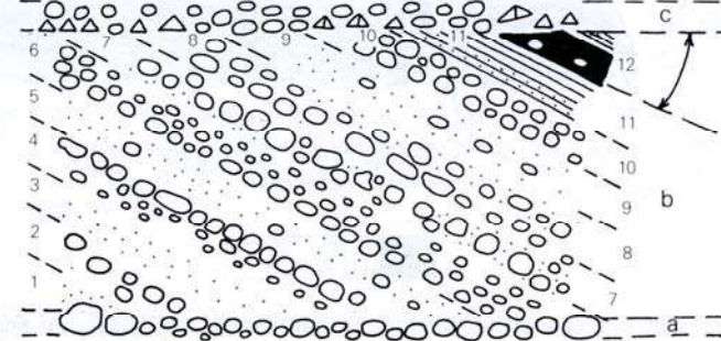
(c) Horizontal and cross stratified beds near the angle of rest
