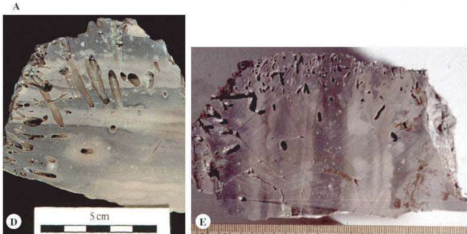
FIGURE 4.10 The Trypanites Ichnofacies. (A) Diagram of the Trypanites Ichnofacies (artwork by Tom Saunders). (B) Entobia in carbonate, Oligocene-Miocene Bluff Formation, Grand Cayman Island. (C) Gastrochaneolites with in situ bivalves ( Zirfaea pilsbyri ), excavated into Triassic sandstones along the margin of the Bay of Fundy, Economy, Nova Scotia. (D),(E) Trypanites excavated into carbonate hardground, marking the Silurian-Devonian disconformity, southern Ontario.
