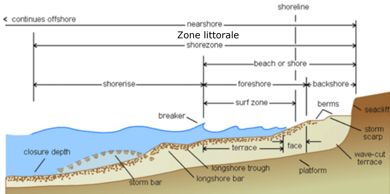
Fig. 410 Schematic representation of the terminology of the various geomorphic units of a beach profile. Various geomorphic features of a beach as well as transition to shelf mud are shown. The terminology is mainly based on EMERY (1960a)
