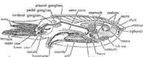
Fig. 1.—Medial longitudinal section of the nautilus and (2) style, showing successive spiral septa and sutures of the two major groups of living cephalopods (from Starr, 1923, p. 82).
