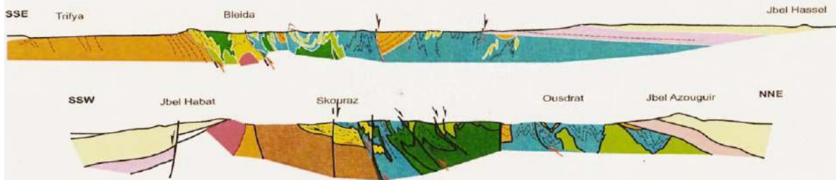
Figure 2: Cross-sections through the Bou Azzer inlier. These cross-sections show clearly the thrusting (in red) of the ophiolites sequence onto the WAC. Some of the major thrusts are reactivated later as normal faults (in black). (modified after Leblanc, 1981)
