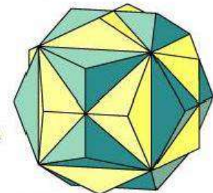
Pyritoèdre [011]
