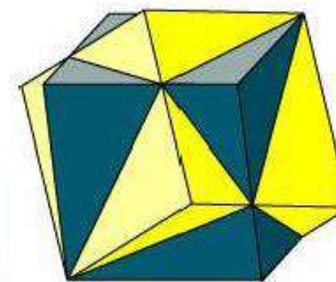
Fluorine [111]
