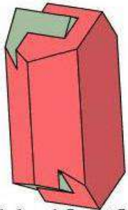
Carlsbad [001]
