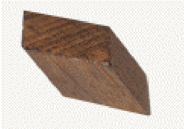
RHOMBOHEDRIQU
