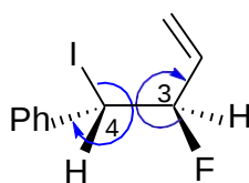
G (3R,4S)
