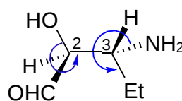
H (2S,3R)
